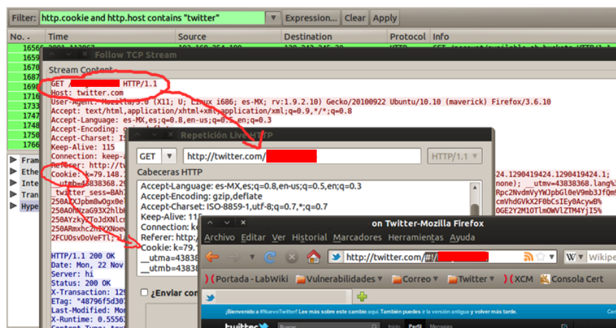
Figura 32- Stealing Twitter Cookies
