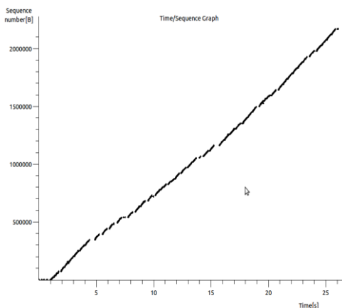
Figura 46- Graph Steven
