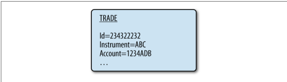
Figure 2-1. Message Composition
