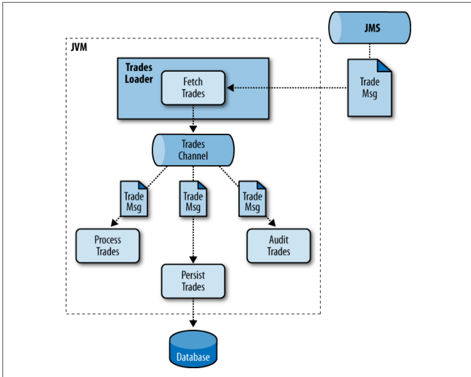
Figure 1-2. Standalone Messaging
