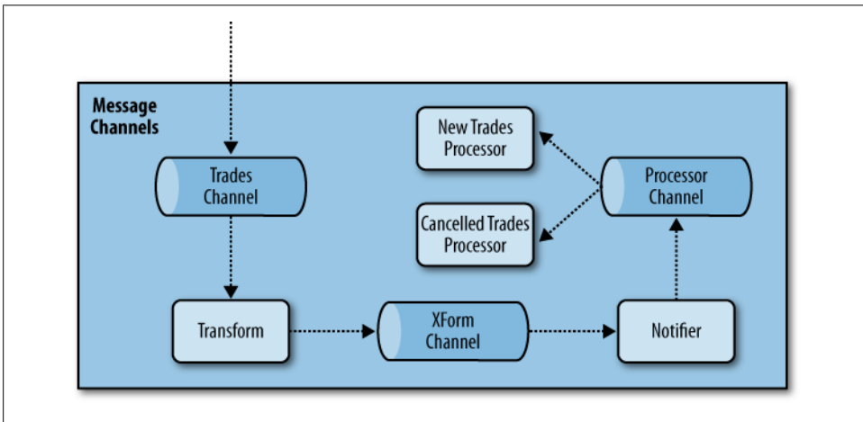
Figure 2-2. Message Channels
