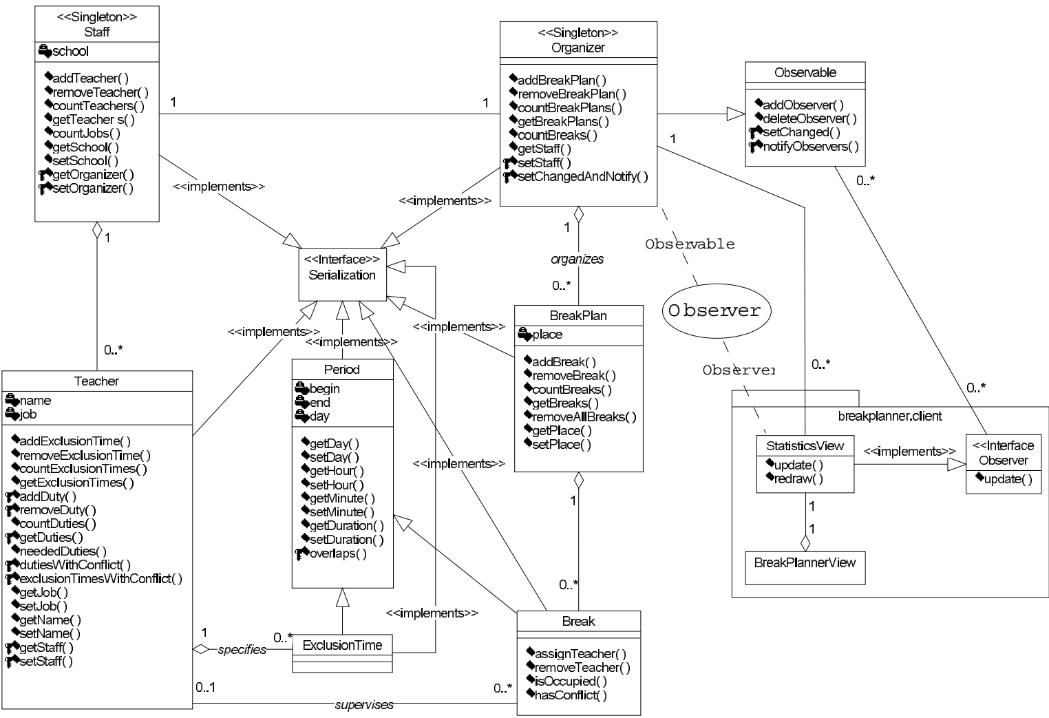
Figure 10: Business-Oriented Design Class Diagram
