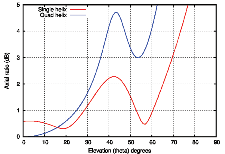
Figure 16: Comparison of the axial ratio performance of the monofilar and quadrifilar helical antennas. Elevation angle is defined such that 0° lies along the axis of the helix.
